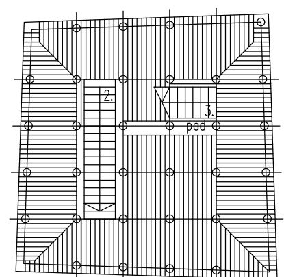
2. emelet +6.00
