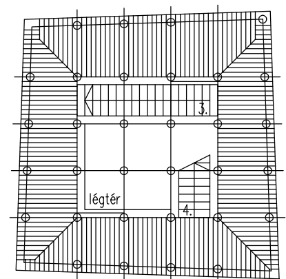
3. emelet +9.00
