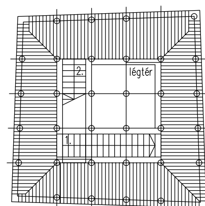
1. emelet +3.00
